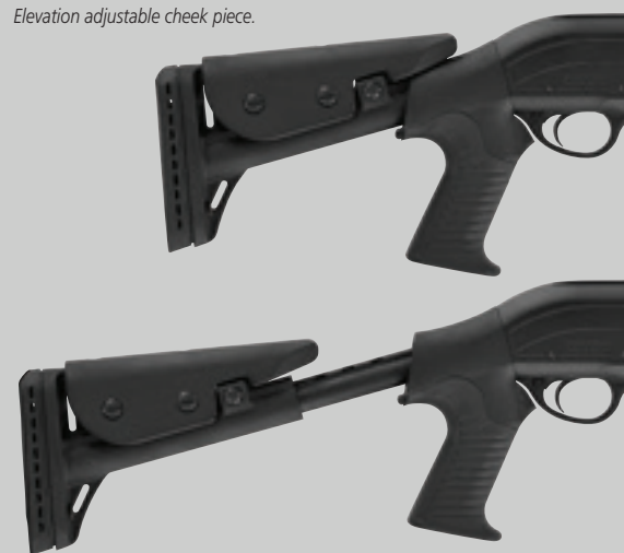
Hatsan design telescopic stock. Stock can be shortened by 10cm (4").
